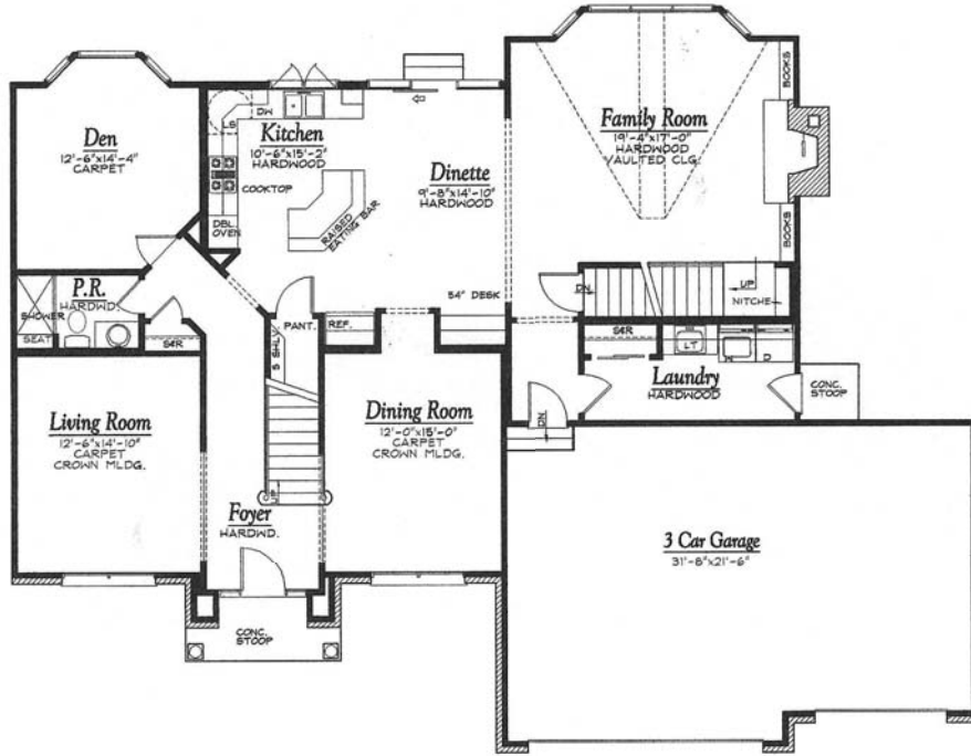
First Floor Plan - 1702 SQUARE FEET
