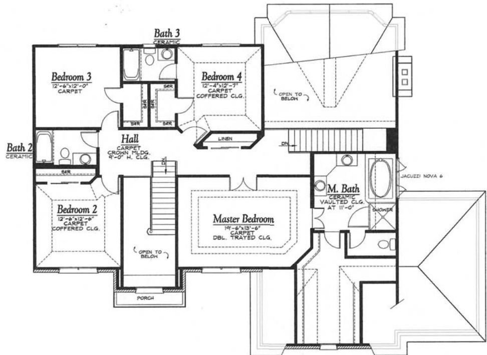
Second Floor Plan - 1461 SQUARE FEET
